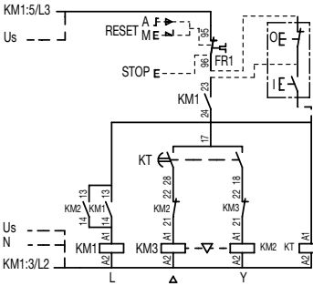
AX06 ... AX205 contactors
